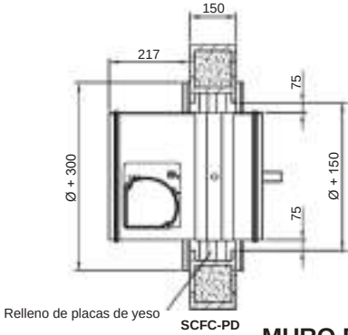
MURO FLEXIBLE
